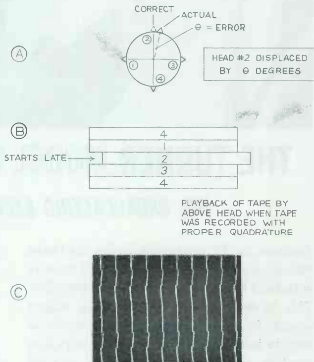
Fig. 15—Space distortion with head quadrature error.
