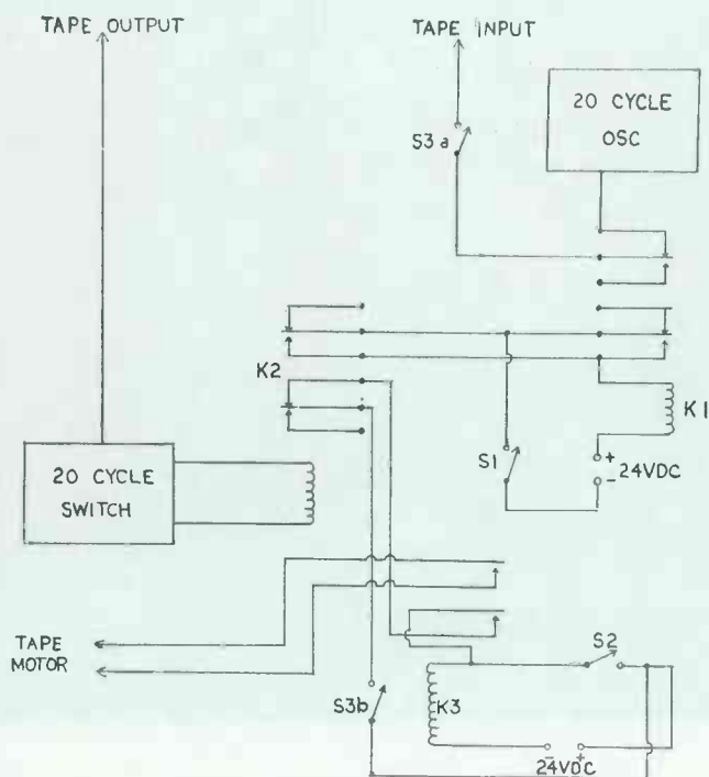
Fig. 1—Relay wiring.
