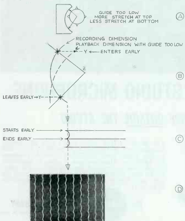
Fig. 14—Space distortion with vacuum guide too low.
